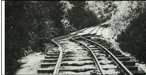
Figure 3-7. Damage to the railroad track between Wrights Station (near the tunnel) and Alma caused by the 1906 earthquake. Both historic settlements and the rail line no longer exist. The gravel road now follows the rail path. The photograph is from the Lawson Report.
